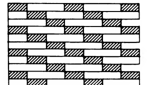
12 1 header; 1 stretcher alternating coursewise with 1/2 bond rising left
